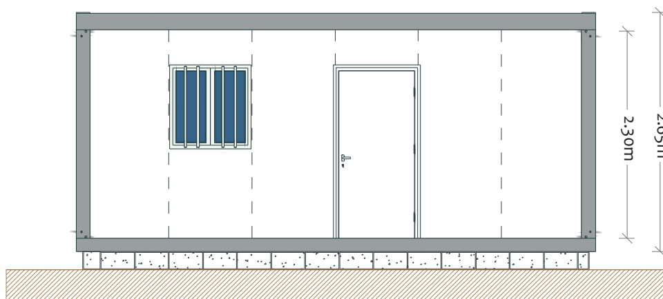
Main Elevation
